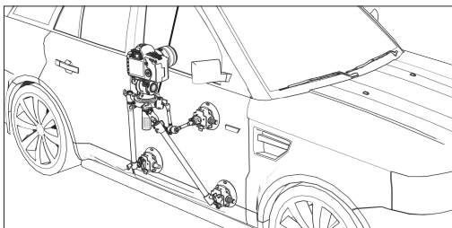
Installation on the vehicle door
